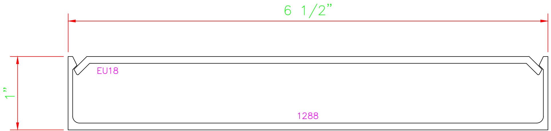
1288 / EU18 6 1/2" X 1" COVER & CLIP
